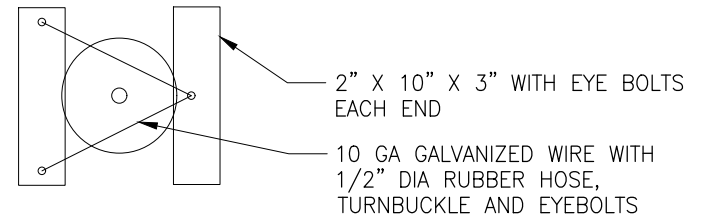
STAKING PLAN
